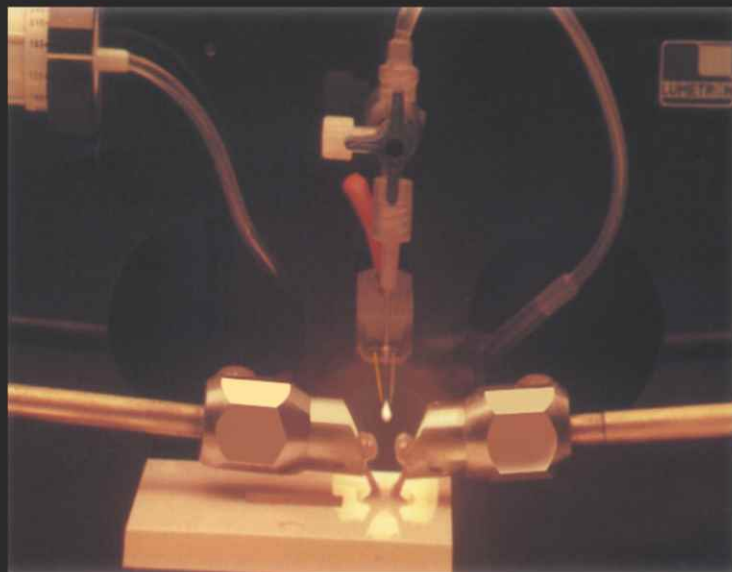
50 drops of 0.1% Ammonium Chloride confirm the non-conductivity
