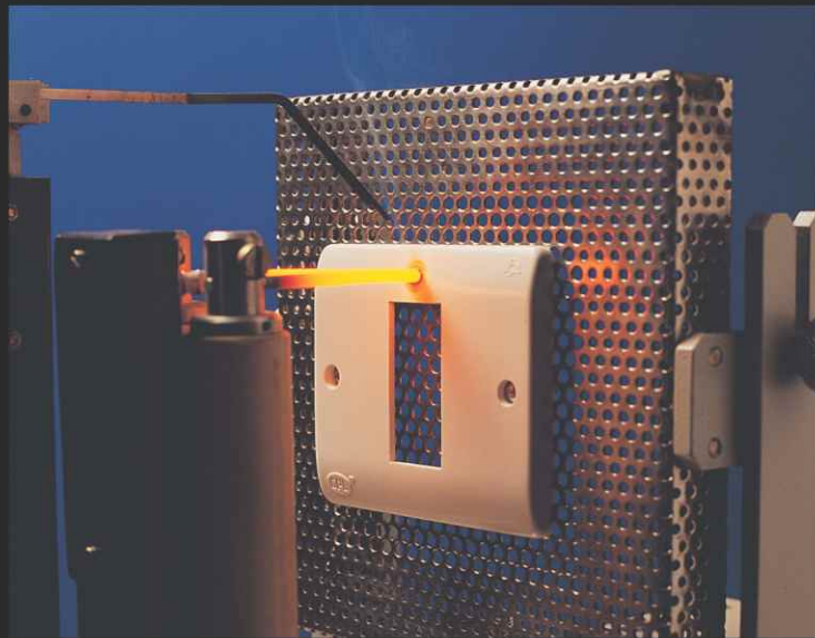
The Glow Wire tests Urea Formaldehyde's fire retarding properties at 850° C
