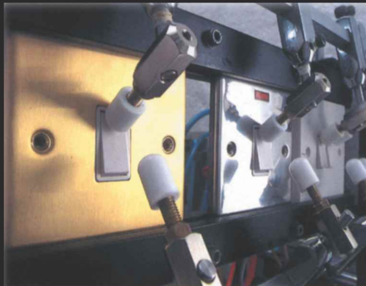
40,000 on-off operations tests the On-load endurance of the switches
